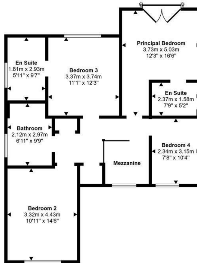
First Floor Approx 76 sq m / 823 sq ft
