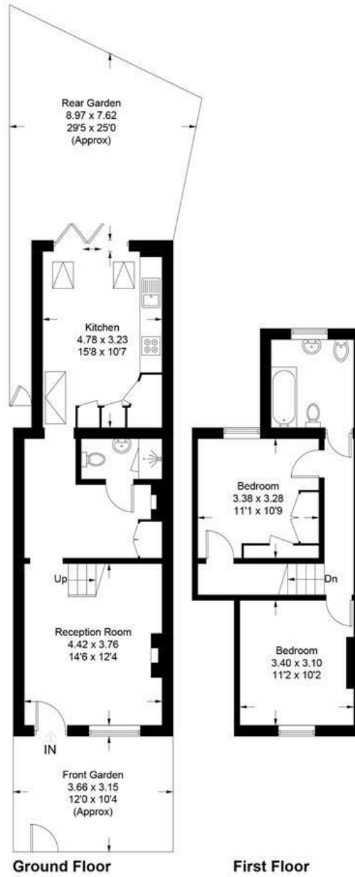
Illustration for identification purposes only, measurements are approximate, not to scale. floorplansUsketch.com © (ID1088857)
