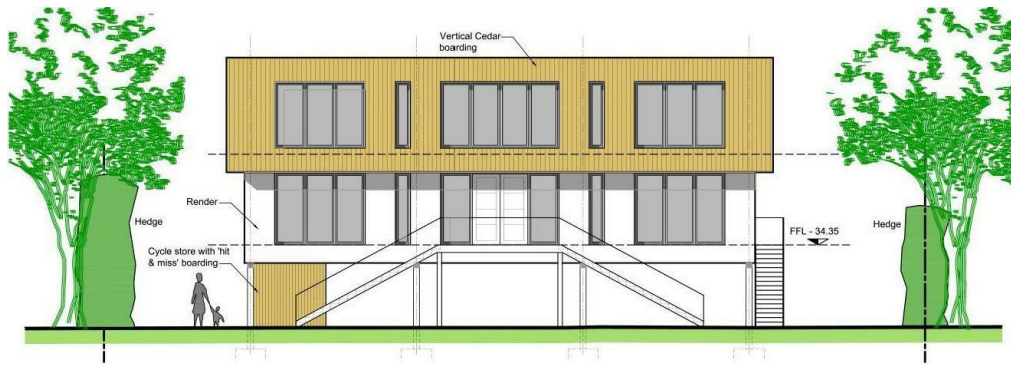
Proposed South East Elevation (Front)
