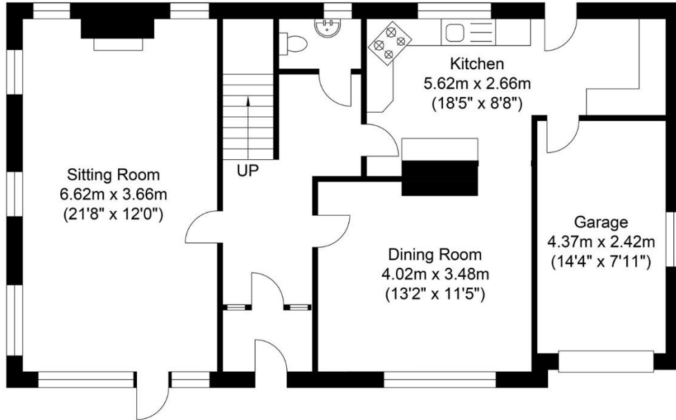
Ground Floor Approximate Floor Area 852.17 sq ft (79.17 sq m)
