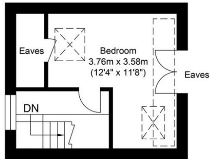
Second Floor Approximate Floor Area 180.83 sq ft (16.80 sq m)
