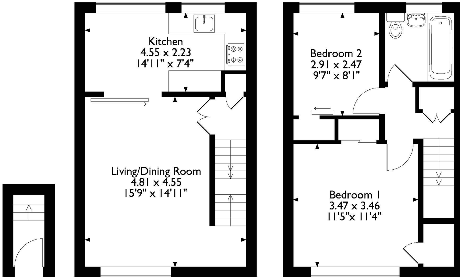
Ground Floor
