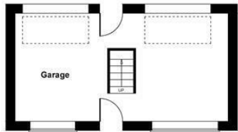
GARAGE GROUND FLOOR
