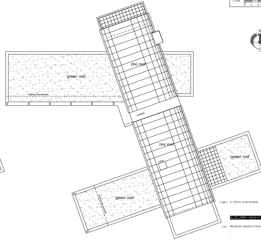
ROOF PLAN 1:100
