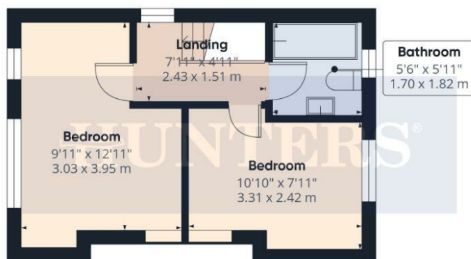
Floor 1
