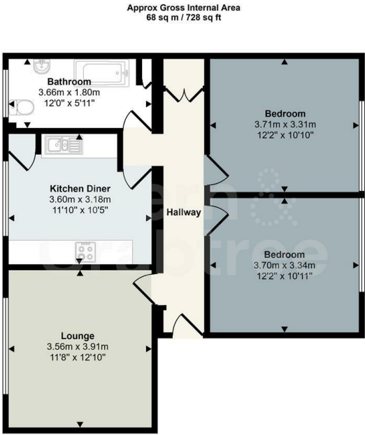
Floorplan
