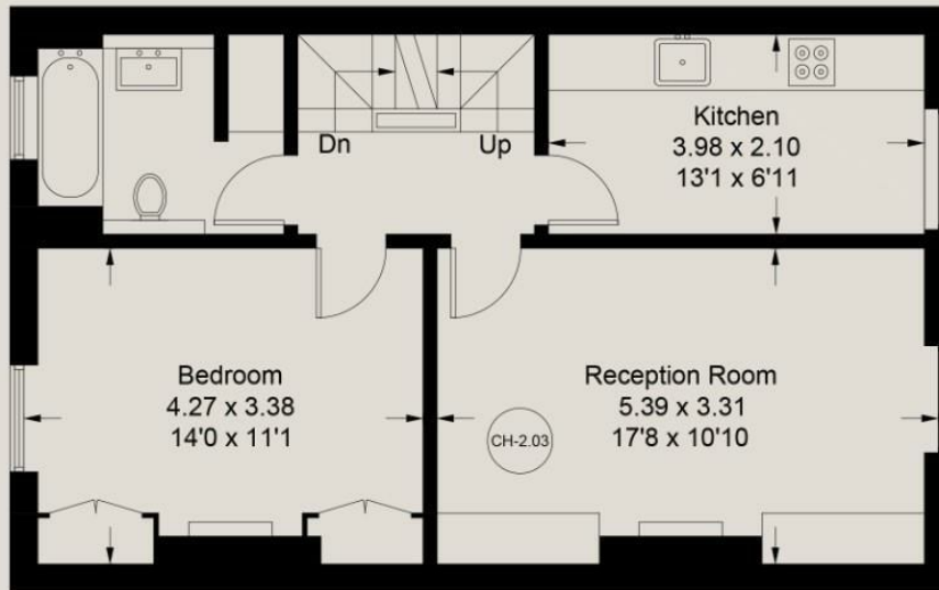
Third Floor
