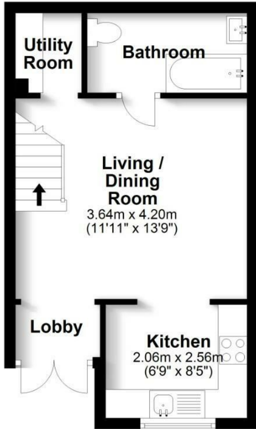
Floor Plan Approx. 29.6 sq. metres (318.2 sq. feet)
