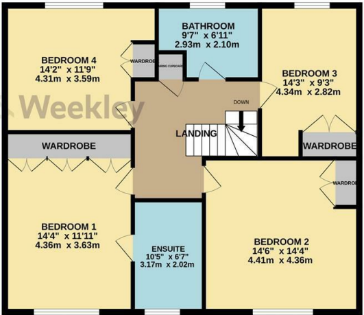
TOTAL FLOOR AREA : 2179 sq.ft. (202.4 sq.m.) approx.
