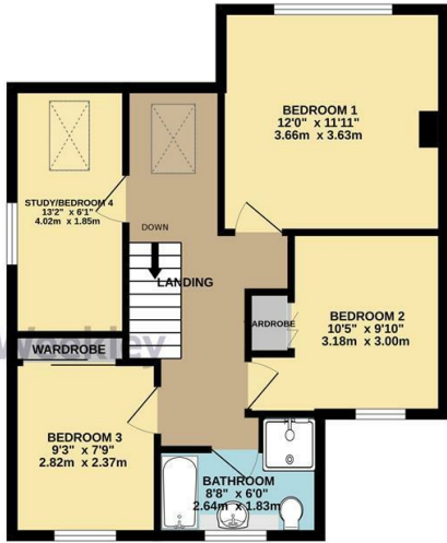
1ST FLOOR 556 sq.ft. (51.7 sq.m.) approx.
