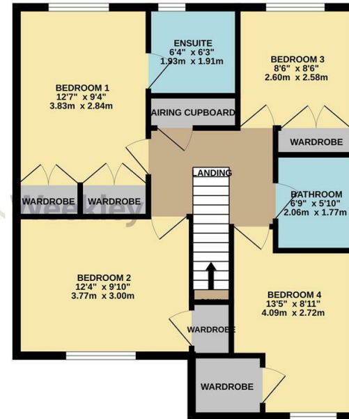
TOTAL FLOOR AREA: 1325 sq.ft. (123.1 sq.m.) approx.
