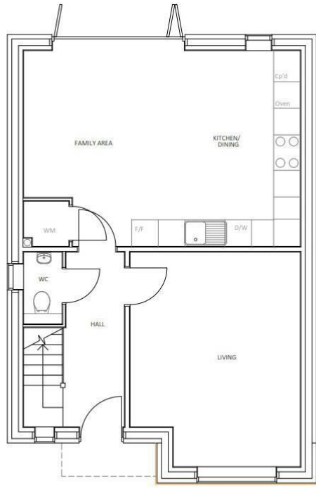
GROUND FLOOR - Plot 15 & 24
