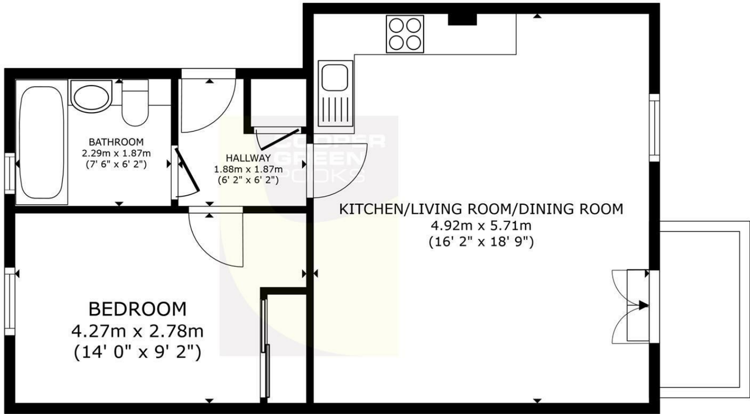
FLOOR PLAN
