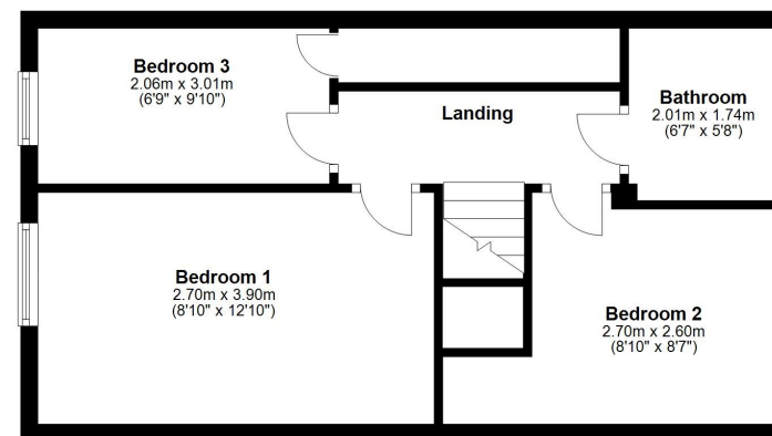
First Floor Approx. 38.8 sq. metres (417.8 sq. feet)
