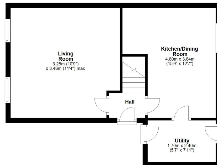
Ground Floor Approx. 38.2 sq. metres (411.5 sq. feet)
