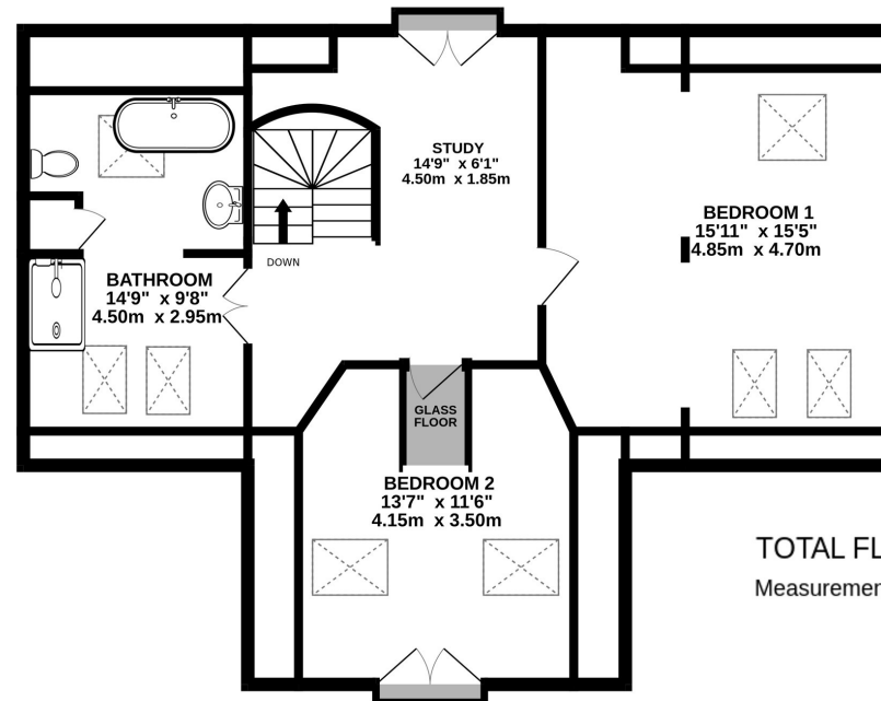
FIRST FLOOR 870 sq.ft. (80.8 sq.m.) approx.
