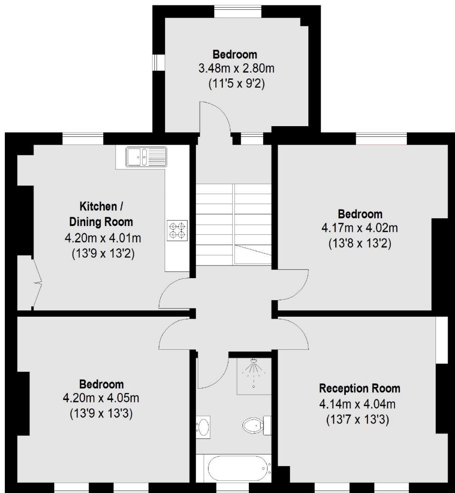
First Floor
