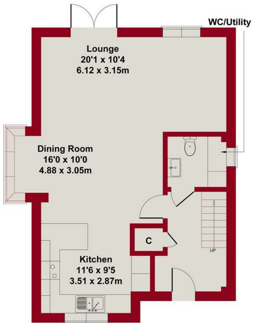
GROUND FLOOR
