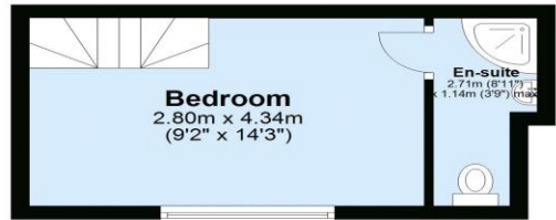
Second Floor Approx. 15.2 sq. metres (163.1 sq. feet)
