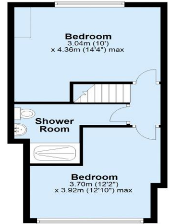
Second Floor Approx. 36.5 sq. metres (393.0 sq. feet)
