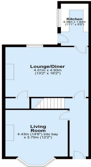
Ground Floor Approx. 49.4 sq. metres (531.6 sq. feet)
