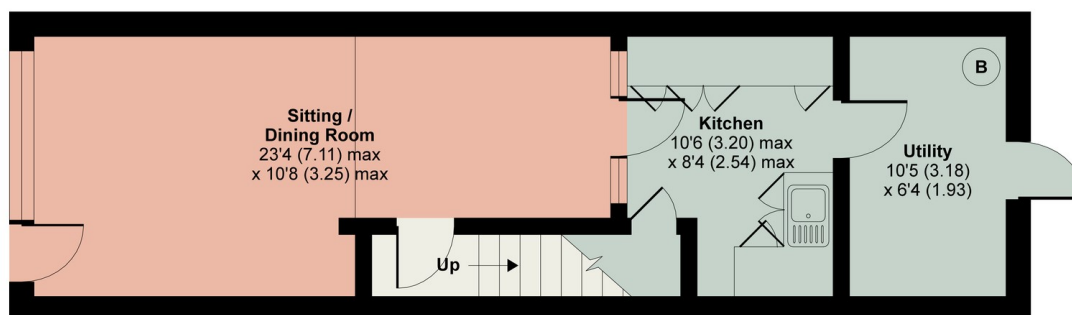
GROUND FLOOR
