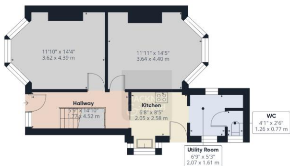
Floor 0 Building 1
