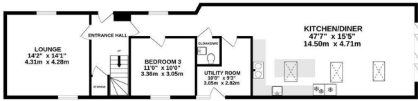
GROUND FLOOR 1007 sq.ft. (93.6 sq.m.) approx.
