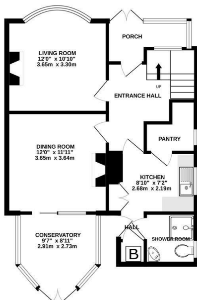
GROUND FLOOR 634 sq.ft. (58.9 sq.m.) approx.
