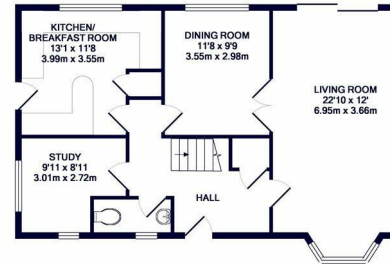
GROUND FLOOR APPROX. FLOOR AREA 729 SQ.FT. (67.8 SQ.M.)
