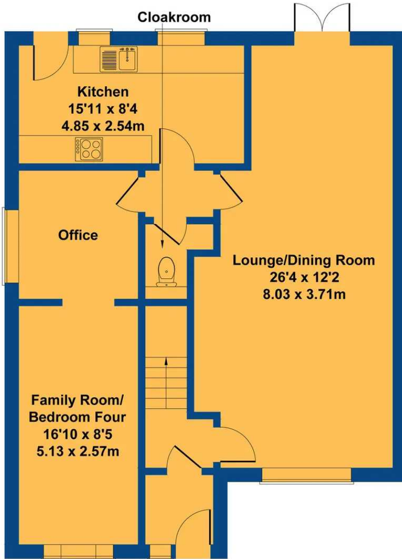
GROUND FLOOR
