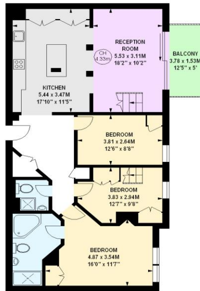
Fifth Floor
