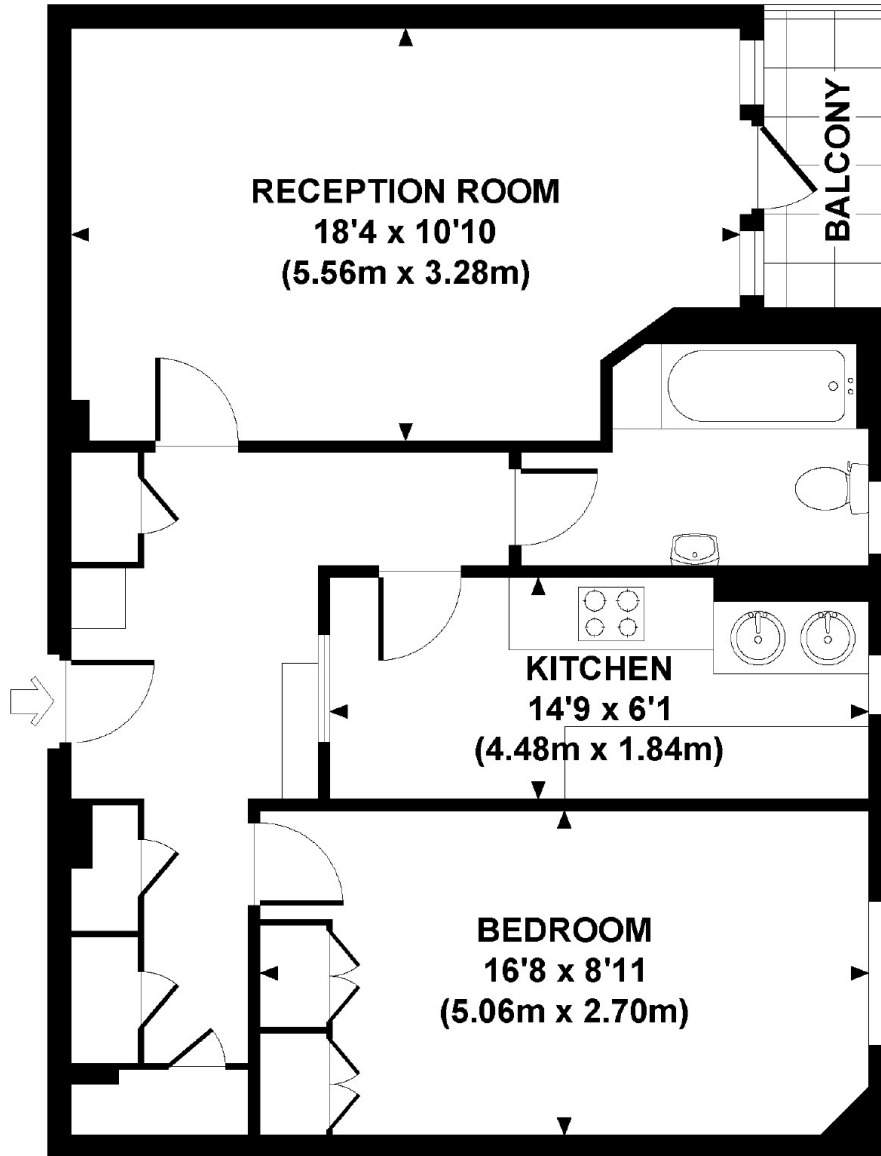
FIRST FLOOR
