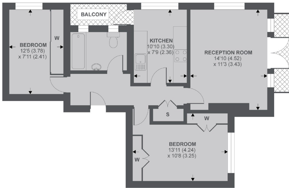
1st Floor
