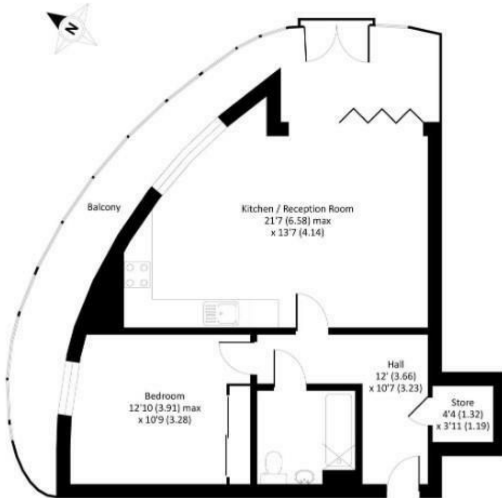
TWENTY-SECOND FLOOR
