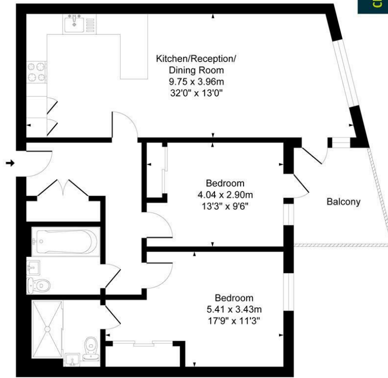
First Floor
