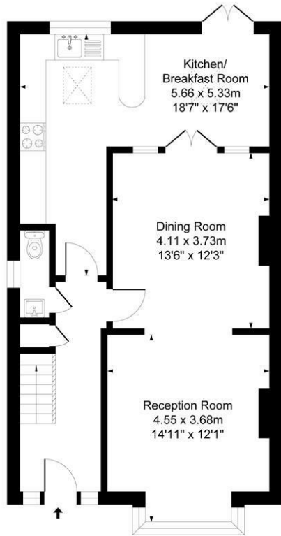
Ground Floor Approximate Floor Area 694.03 sq.ft (64.47 sq.m)
