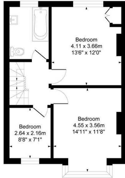
First Floor Approximate Floor Area 517.57 sq.ft (48.08 sq.m)
