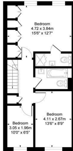
Second Floor Approximate Floor Area 529.58 sq.ft (49.19 sq.m)
