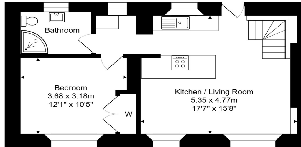
Ground Floor Area: 45.2 m 2 ... 486 ft 2
