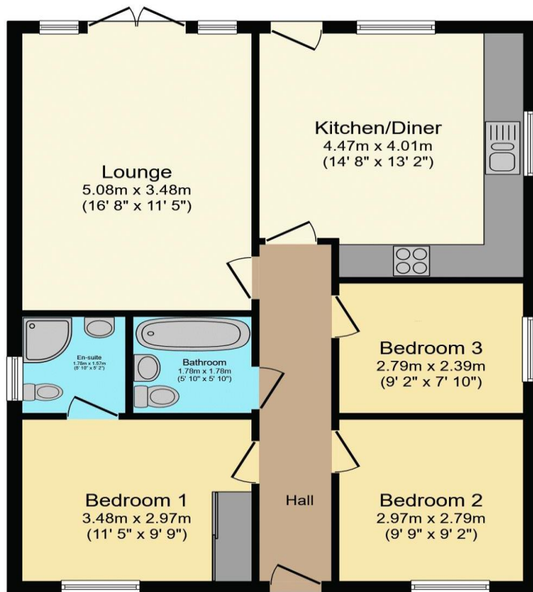
Floor Plan
