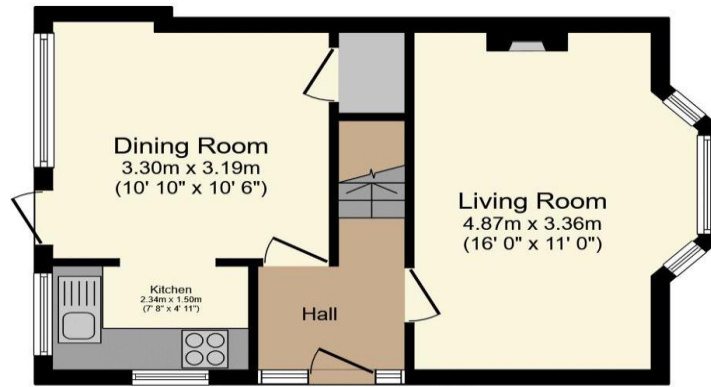
Floor area 36.1 m 2 (389 sq.ft.) approx
