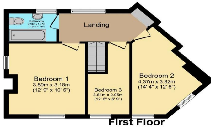
Floor area 41.5 m 2 (447 sq.ft.) approx
