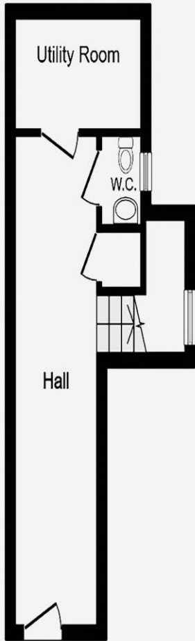
Ground Floor
