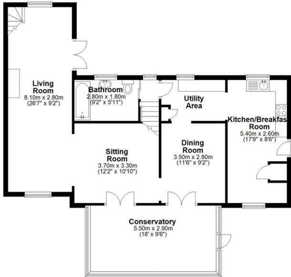
Ground Floor Main area: approx. 90.9 sq. metres (978.3 sq. feet) Plus outbuildings: approx. 23.9 sq. metres (256.9 sq. feet)
