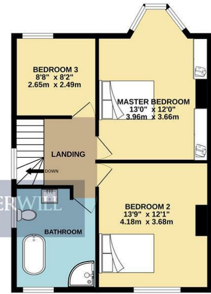
FIRST-FLOOR 575 sq.ft. (53.4 sq.m.) approx.
