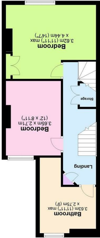
First Floor Approx. 43.2 sq. metres (465.4 sq. feet)
