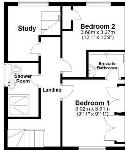
First Floor Approx. 36.9 sq. metres (396.9 sq. feet)
