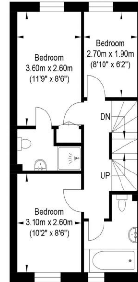
First Floor Approximate Floor Area 414.84 sq ft (38.54 sq m)
