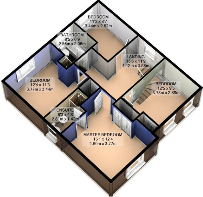
1ST FLOOR APPROX. FLOOR AREA 741 SQ. FT. (68.8 SQ. M.)
