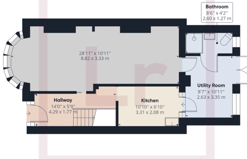
Ground Floor
