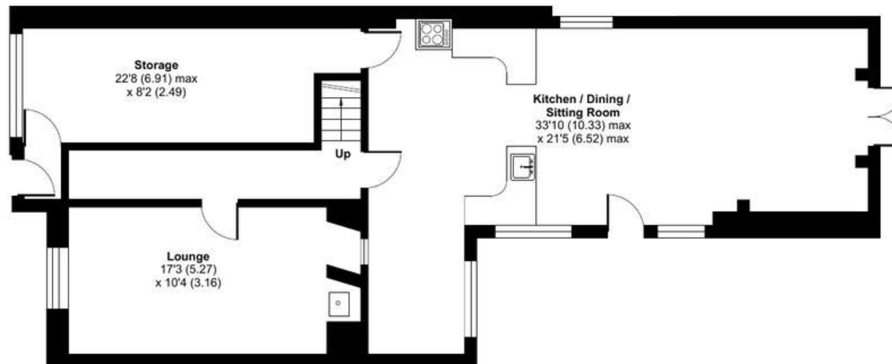
GROUND FLOOR
